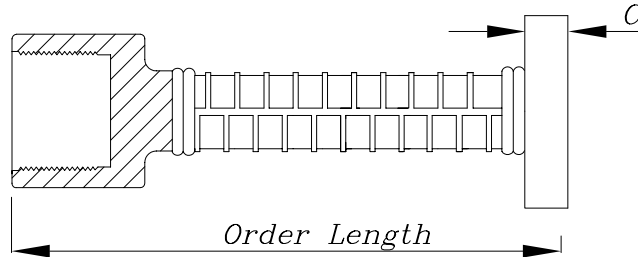
HRC 520 / 120 (Headed)
